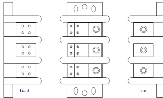
Figure 5 Main Power Terminal Block
