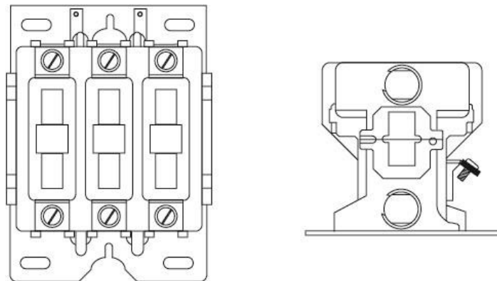
Fig. 7. Magnetic Contactor
