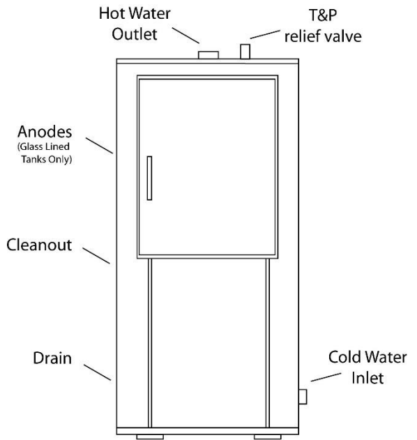
Fig. 3. Water Connections
