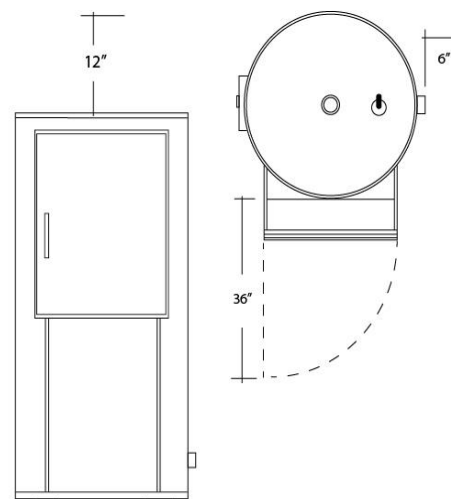
Fig.2. Clearances from Combustible Construction
